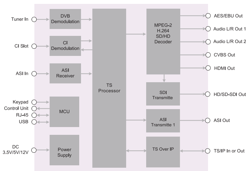
DMM-1520P Functional Block Diagram
