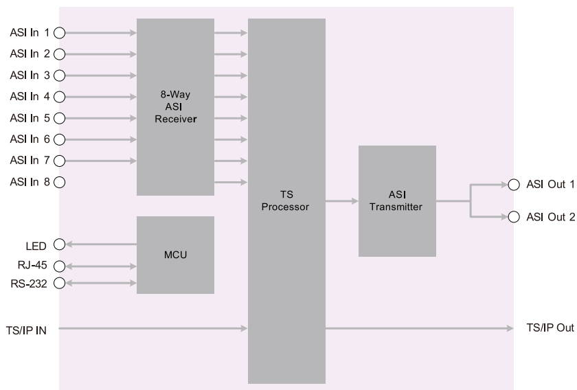
DMM-1400MX Functional Block Diagram
